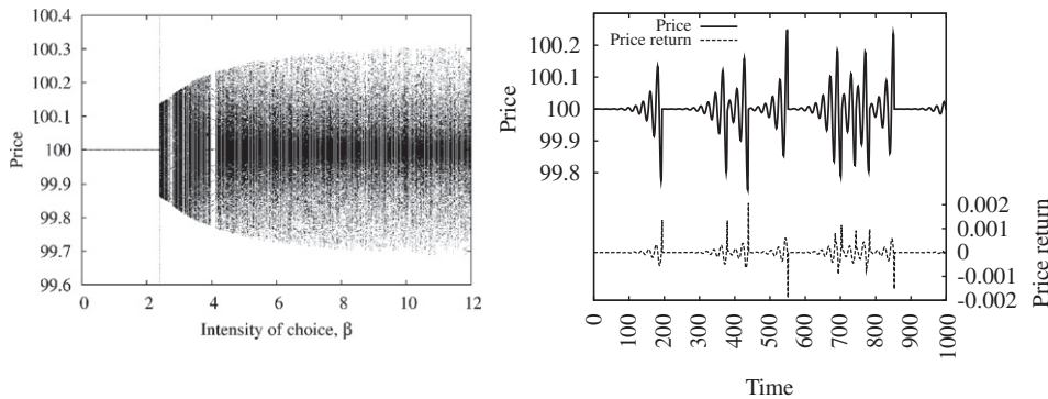
Fig. 1. Bifurcation diagrams for the WA under the LML. For each \beta \in (0, 12) , 300 points after 10 000 transitory periods are shown. Left panel: Neimark–Sacker bifurcation of fundamental steady state. Parameters are: r = 0.1 , \bar{y} = 10 , \nu = 0.1 , g = 1.2 , and C = 1 . Right panel: Time series of the price and return with random dividend and small dynamic noise. Both noise terms are i.i.d. normal with standard deviation equal to 0.005.
